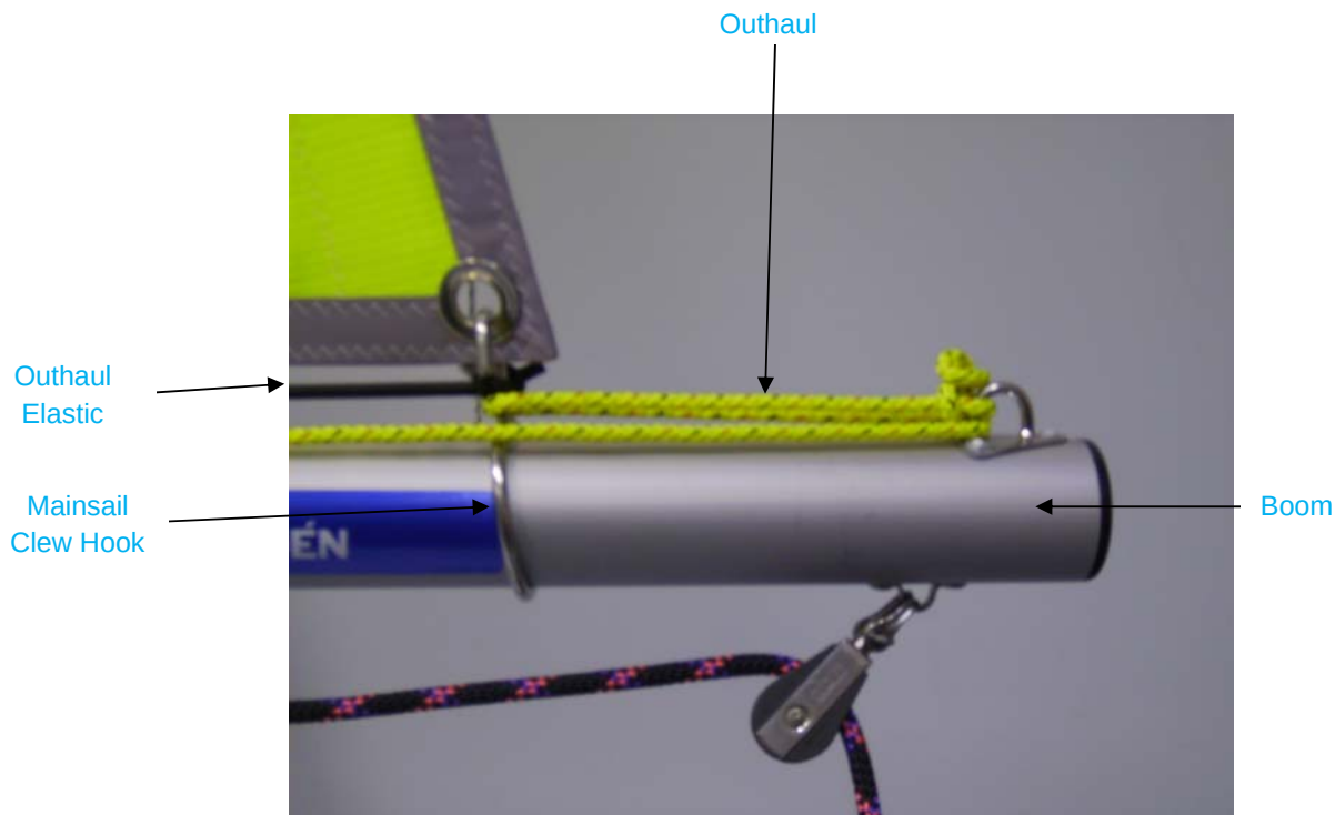
Picture 4.12 The Aft End of the Boom
