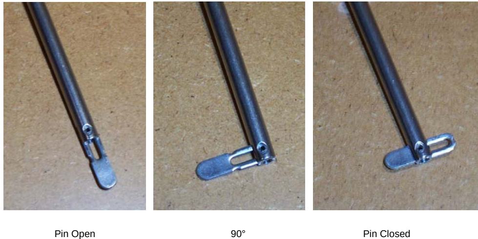
Picture 4.8 The Mast-Gate Pin
